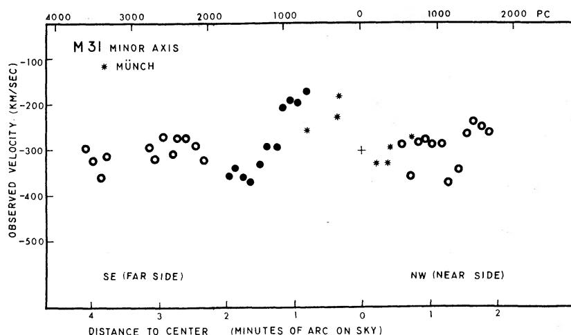
FIG. 8.—Observed velocities along the minor axis of M31, measured from the [\text{N II}] \lambda 6583 emission line. Different symbols represent different plates. Cross at R = 0 , V = -300 km sec -1 marks the systemic velocity of the galaxy. Stars indicate the velocities measured by Münch (1960) from the [\text{O II}] \lambda 3727 emission line.
